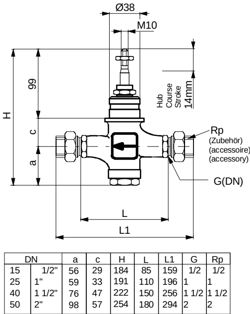
Dimension drawings 7M100 V6R
