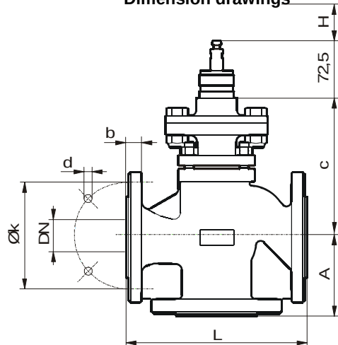
Dimension drawings
