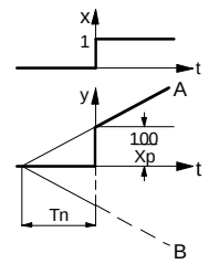
PI-controller
