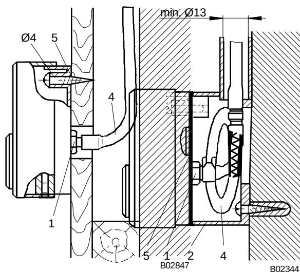
Panel fitting
