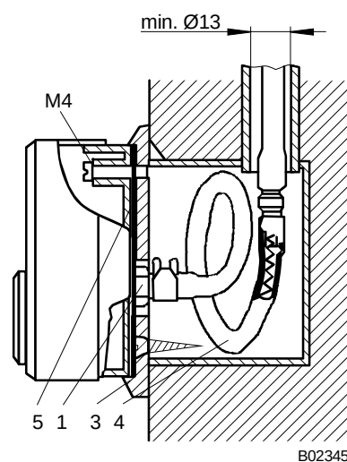
Recessed fitting
